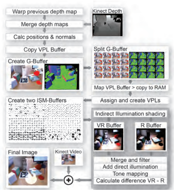
Figure 2: This figure shows the algorithm outline. The raw depth values from the Kinect sensor are preprocessed to improve the quality of the real scene reconstruction. Furthermore a G-Buffer is created and afterwards split to reduce shading costs. The primary light sources generate VPLs from which ISMs are created. The VR- and R-Buffers are created in parallel, while the shading computation is performed only once. After some finishing steps like merging, adding direct illumination and tone mapping, the video frame is added to the difference between the VR- and R-Buffers.
