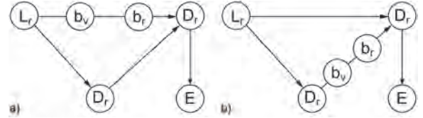
Figure 4: Illustration a) and b) show situations where naive shadow mapping cannot handle correct visibility. In contrast to [4], our method is able to correctly evaluate these paths.
