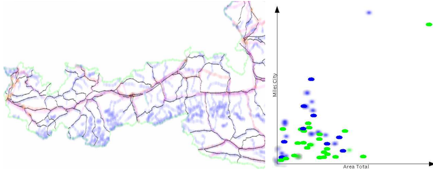
Fig. 14. Two examples of an SDOF visualization: streets standing out of an SDOF map visualization on the left (other parts of the map blurred) and a scatterplot with SDOF effect on the right.
