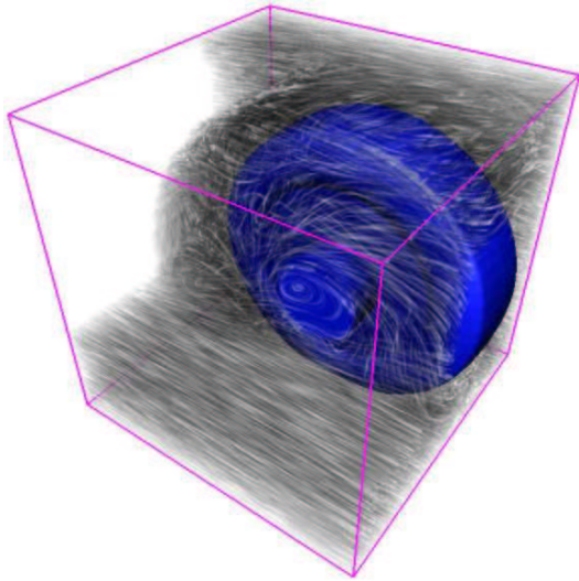
Figure 11: An LIC visualization showing a simulation of flow around a wheel. 59 The appropriate choice of transfer function results in a sparser noise texture. Image courtesy of Rezk-Salama et al. 59
