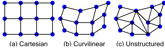
Figure 3: Grids involved in flow simulation – rectilinear (a) vs. curvilinear (b) vs. unstructured grids (c). Issues are implicit (a) vs. explicit locations (b, c), implicit (a, b) vs. explicit neighborhood (c).
