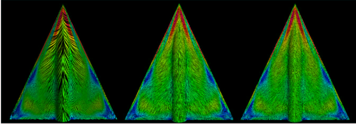
Figure 12: A comparison of 3 LIC techniques: (left) UFLIC 65 , (middle) ELIC 51 , and (right) PLIC 82 . Image courtesy of Verma et al. 82 .
