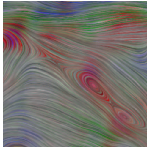
Figure 9: A composite “color woven” LIC image of 2D flow that highlights areas of significant positive vorticity (red), negative vorticity (blue), strongly negative Reynolds shear stress (green), and high swirl strength (orange and magenta). Image courtesy of Urness et al. 76 .
