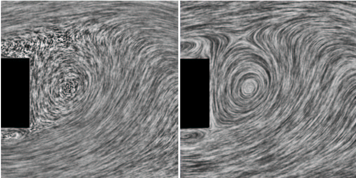
Figure 6: Visualization of flow past a box using (left) spot noise and (right) LIC. Simulation data courtesy of AVL ( www.avl.com ).
